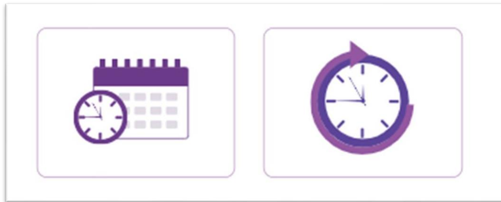
Playlist Selection
